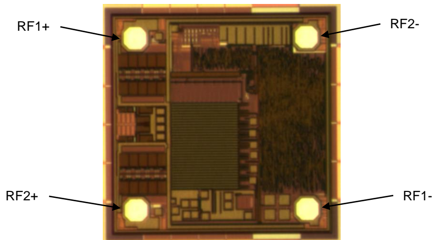
Figure 2-7 Monza 4 tag chip die orientation
