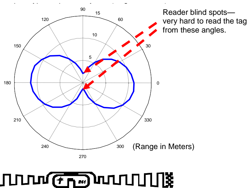
Figure 2-1 Read Range for Monza 4-based, 95 x 8 mm Dipole Tag (Impinj Reference E41)
