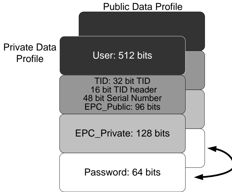
Figure 2-4 Monza 4QT Tag Chip Private Data Profile
