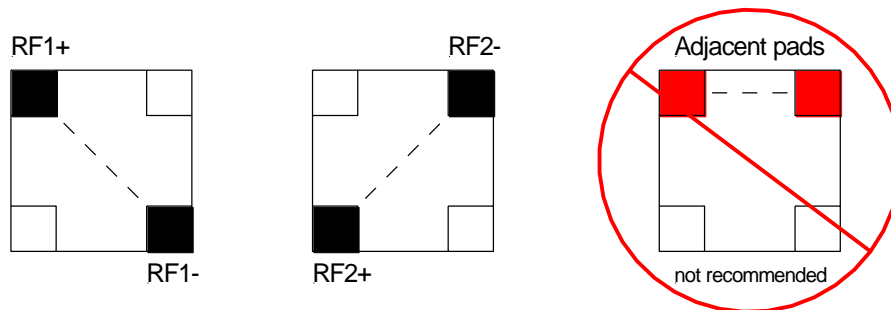
Figure 3-3 Chip/antenna connection possibilities for single-port configuration
